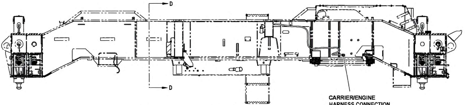
SECTION A-A (AXLES NOT SHOWN FOR CLARITY)
