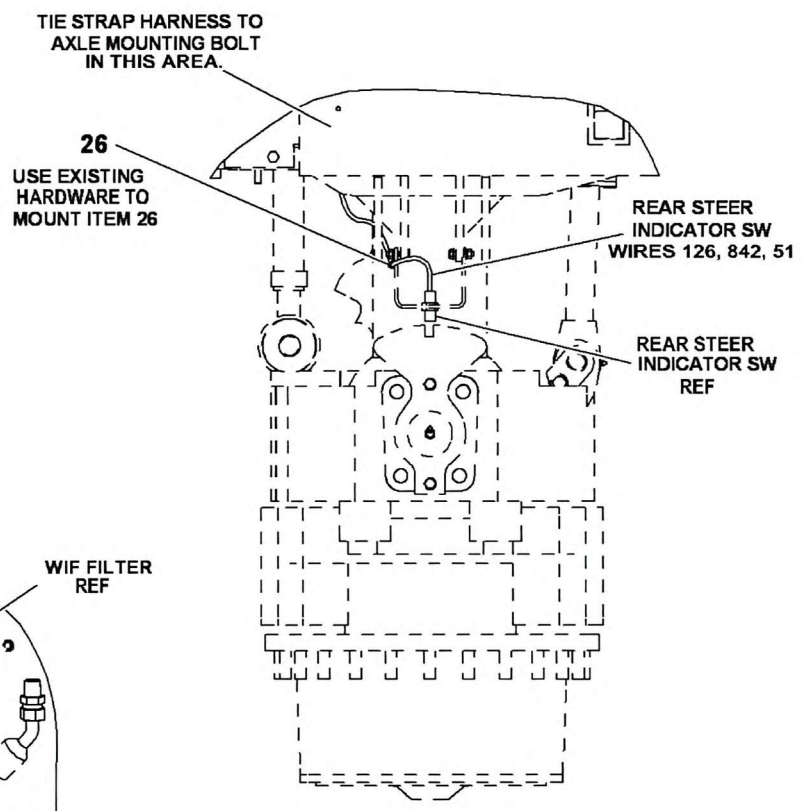
DETAIL J REAR STEER INDICATOR (LEFT REAR WHEEL) (AXLE LOCKOUT CYLINDER NOT SHOWN FOR CLARITY)
