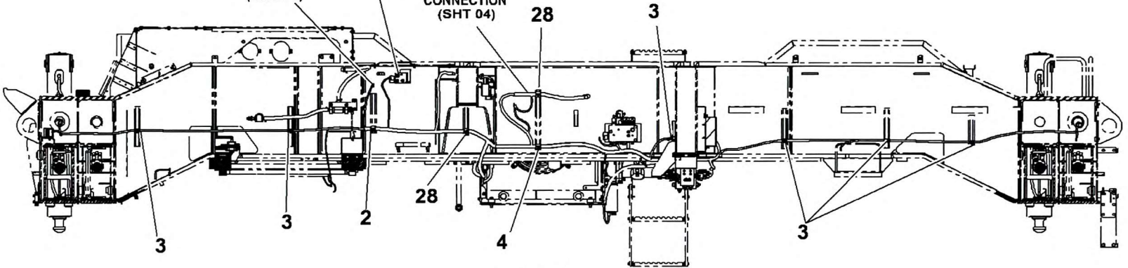
SECTION B-B (AXLES NOT SHOWN FOR CLARITY)
